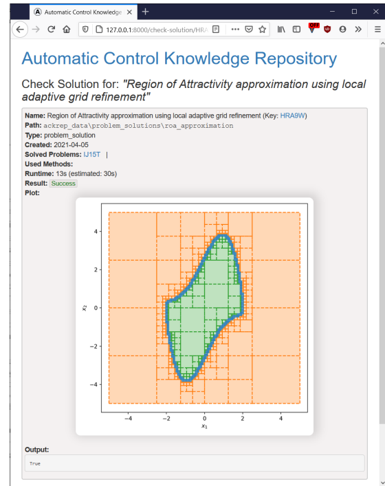
Fig. 6. Screenshot of ackrep_web . Currently displayed is the result page of the check solution command for a region of attraction approximation of the Van der Pol oscillator. The relevant metadata is shown along with the calculation result.
