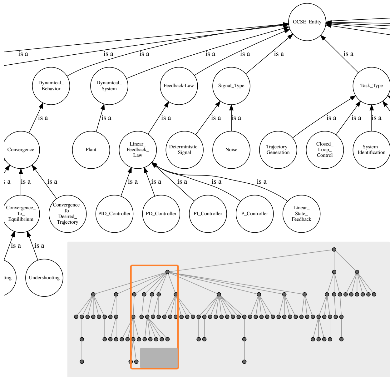
Fig. 3. Section of the taxonomy (subclass hierarchy) of the Ontology of Control Systems Engineering (OCSE). Note that the depicted is_a -relation is only one of several relations between the concepts. The inset in the lower part shows an unlabeled overview of the whole taxonomy graph with the visible section highlighted.
